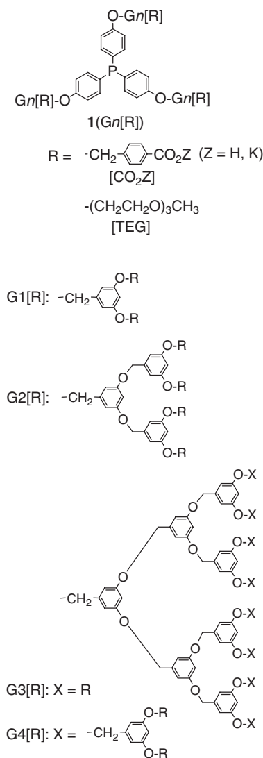
Figure 1. Structural formulas of dendrimer 1 (Gn[R]) and Gn[R] dendrons ( n = 1–4).
