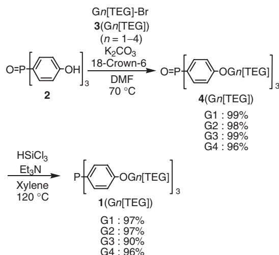
Scheme 1. Synthesis of dendrimer 1(Gn[TEG]) .
